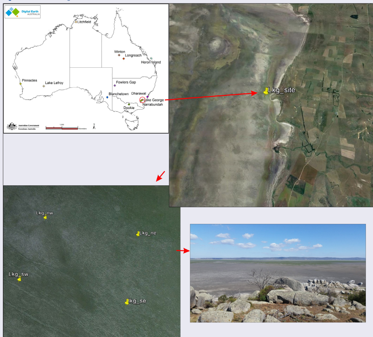
Figure 6.15 Lake George validation site
