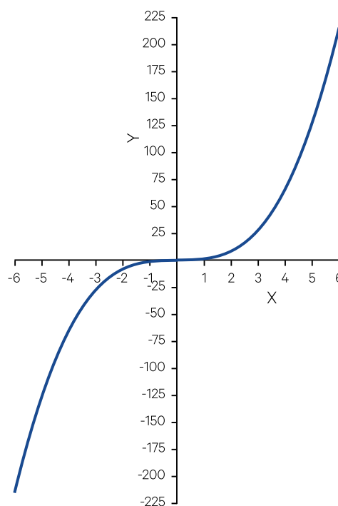
Figure 3.13 Cubic transformation
