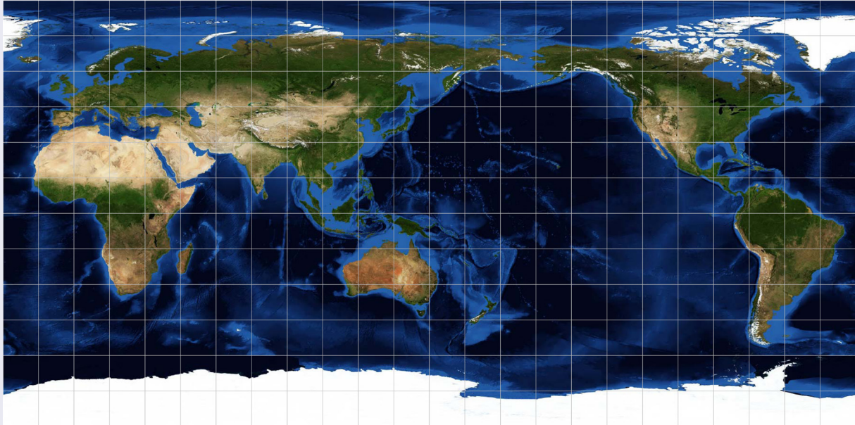
Figure 1.17 Equirectangular or Plate Carrée 'projection'
