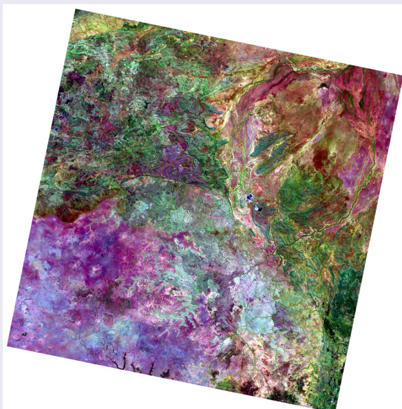
c. Path 100, Row 73, acquired on 6 July 2016
