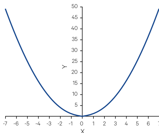
Figure 3.12 Quadratic transformation
