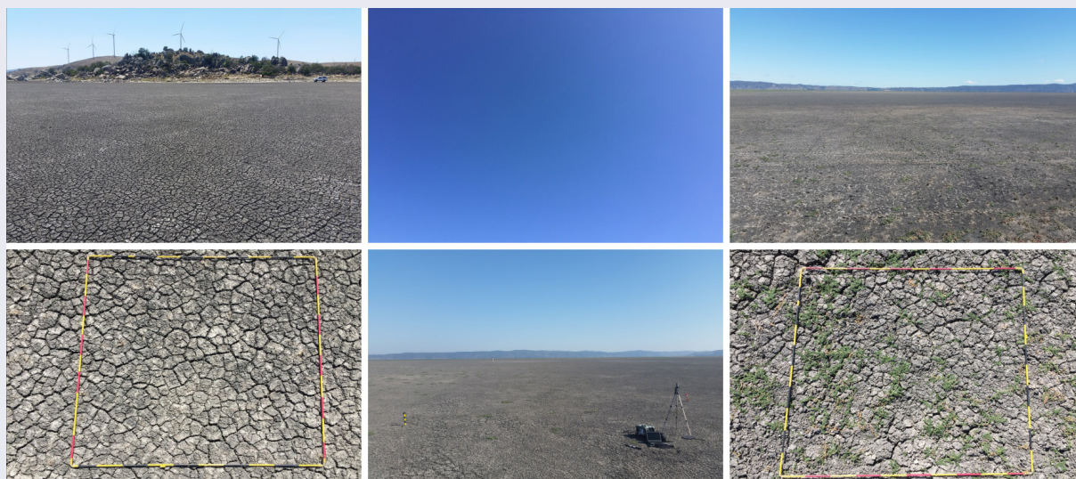
Figure 6.17 Lake George field sampling on 3 May 2018
