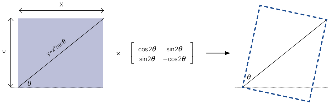
Figure 3.10 Reflection operation
