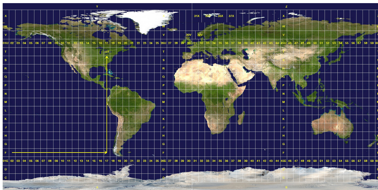
Figure 1.25 Universal Transverse Mercator grid
